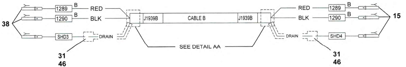
CABLE DETAILS J1939
